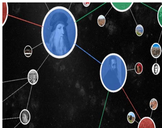
Knowledge Graph
