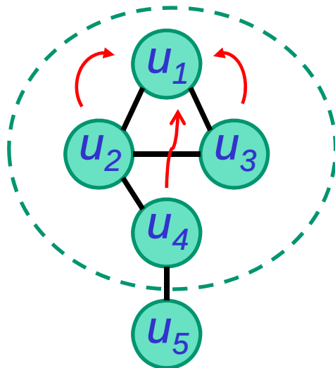
Information Propagation
