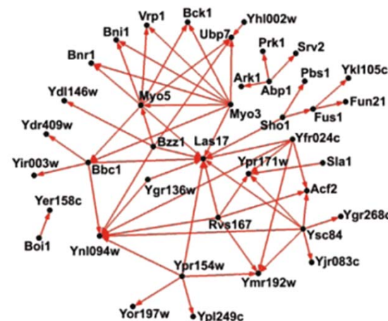
Biological Network
