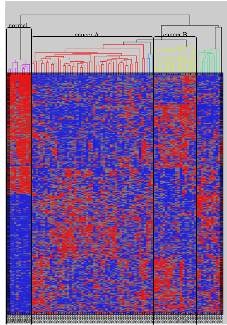
Un-normalized* K-L
