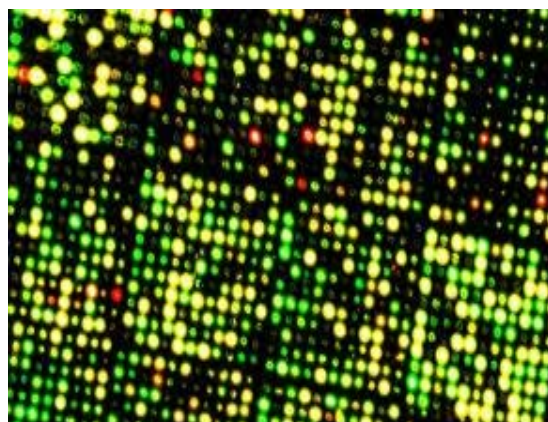
Image Data
