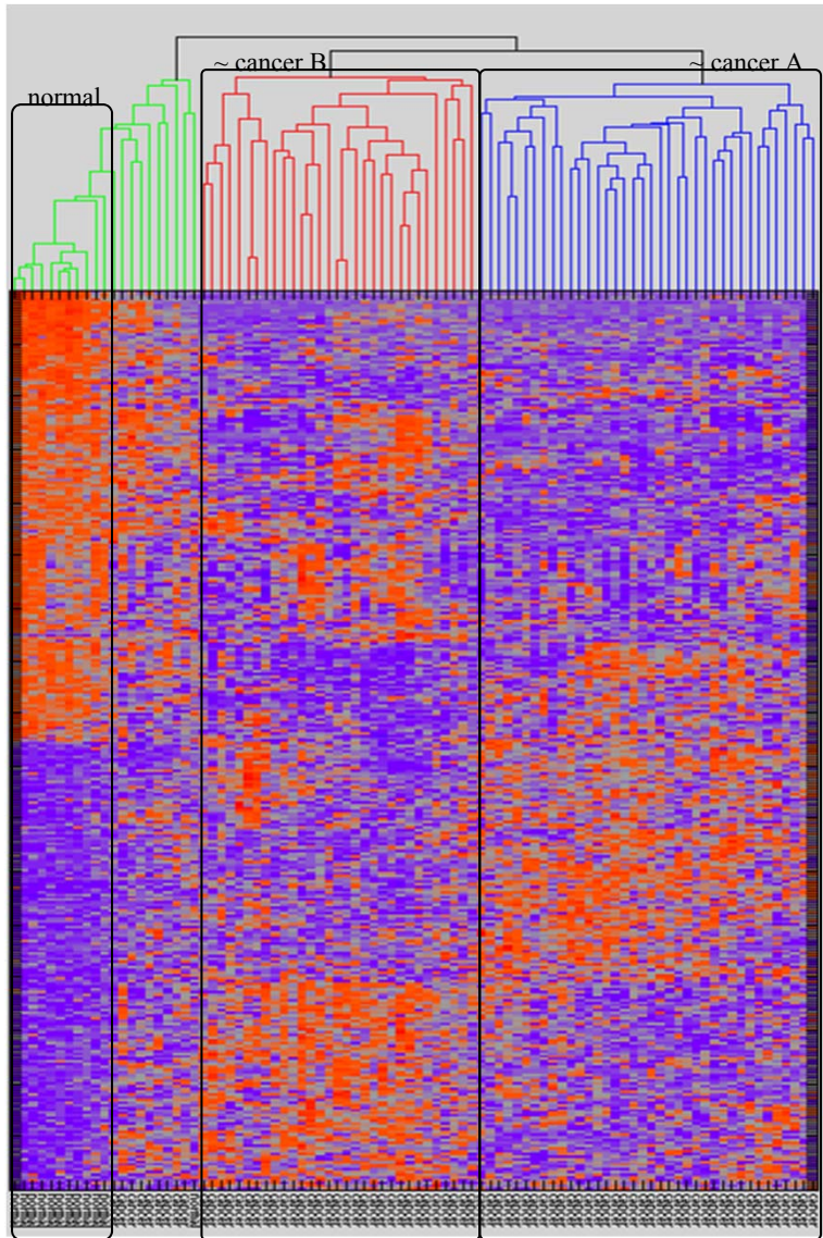
Correlation Coefficient
