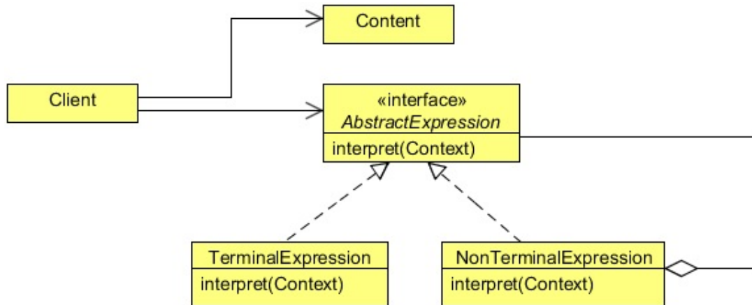
Figure 21.1: - Class Diagram
