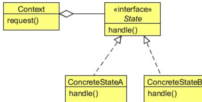
Figure 18.1: - Class Diagram
