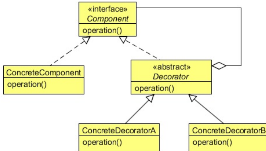
Figure 22.1: - Class Diagram
