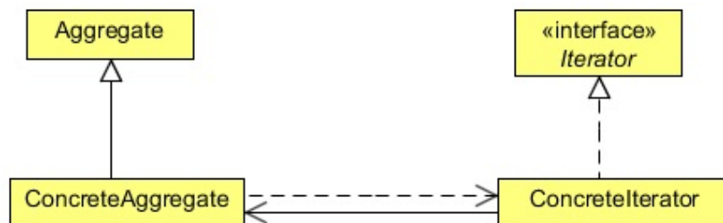
Figure 23.1: - Class diagram
